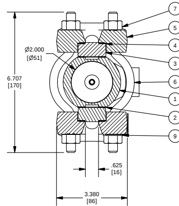
SECTION X-X SERIES TTLCH-10
