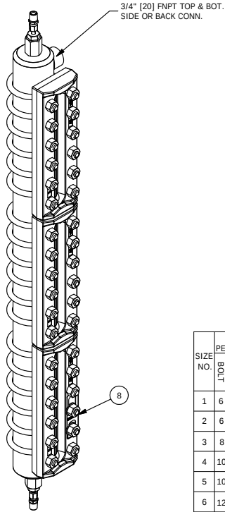
REFLEX GAGE RTLCH-10
