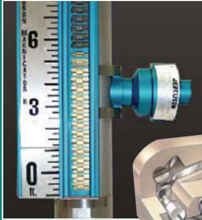
Cutaway view
