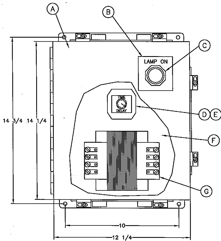
ASSEMBLY VIEW
