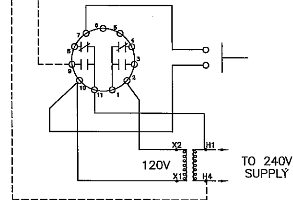
INTERWIRING DIAGRAM
