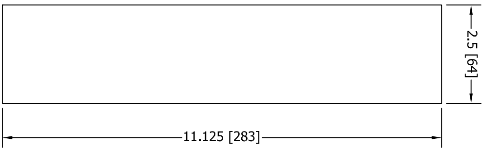
PANEL CUTOUT
