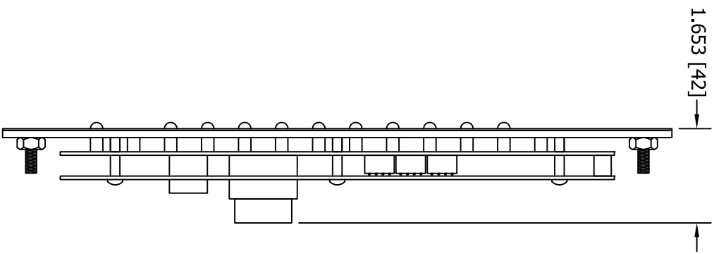
SIDE VIEW
