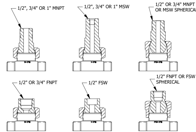
GAGE CONNECTION (3/4" FSW UNION CONNECTION NOT AVAILABLE AS STANDARD)
