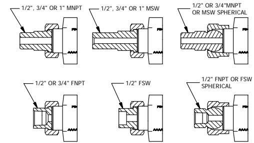
TANK & GAGE CONNECTION
