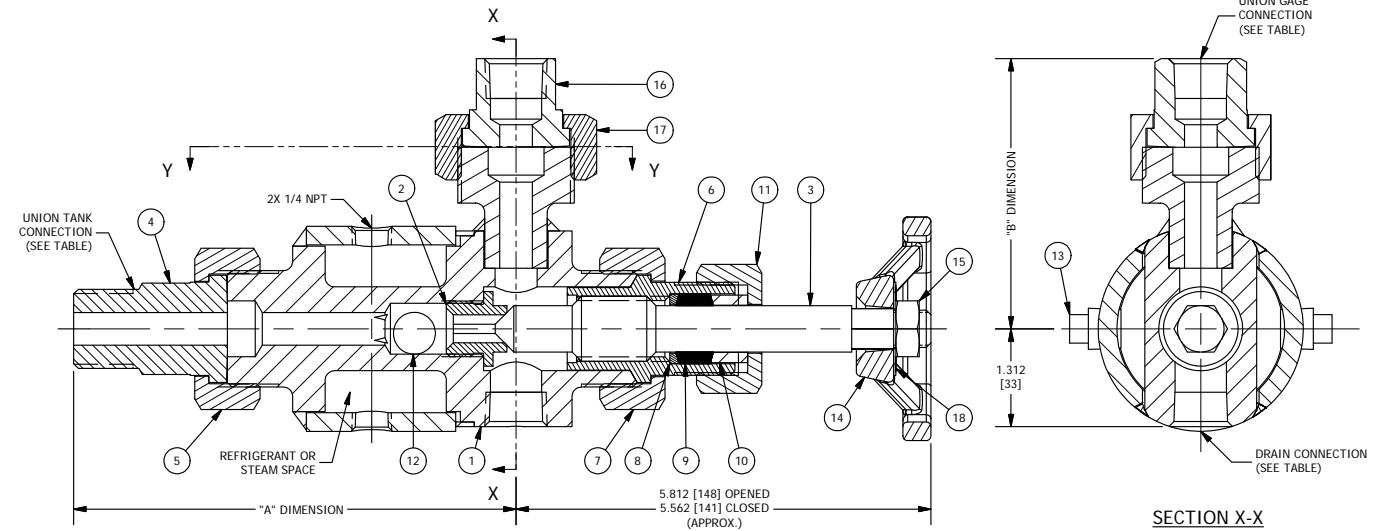
SECTION Y-Y
